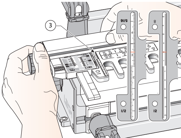
7-5 Add dimensions ① and ②. Set the router stop fence to this total on the fence scale ③ at both ends of the template. Tighten the fence knobs. If your router base is small, see 7-6 below.
