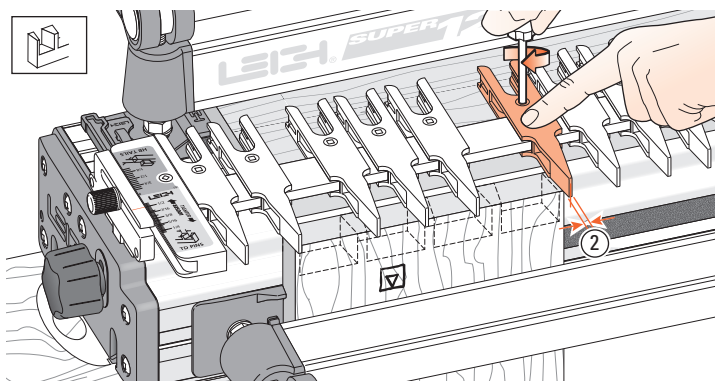
8-12 Leave three guidefingers over the board. Lock the right-most guidefinger with its center-line about \frac{1}{8} " [3mm] ② in from the right edge of the board to form the other half-pin. Judge this distance by eye: it need not be exact. The sockets and pins will align automatically.
