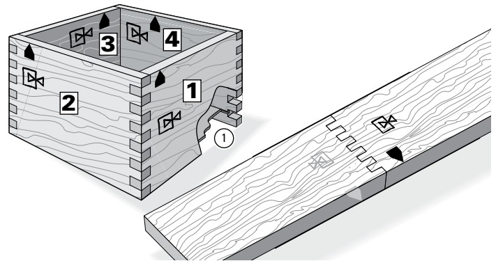
6-16 Keeping the marked side stop edges of all boards toward the top (or bottom) of the box, select the preferred outside faces before marking and routing the grooves 1 for the box bottom. Remember, box joint corners need clamping from both directions, or use strap clamps and blocks. The same method will produce square end-on-end joints. ■
