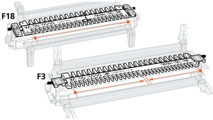
3-1 The active comb (the one you wish to use) is positioned toward you at the front of the jig. Depending on the Template model and comb size selected, the active comb may start at either the right, or left-hand side of the jig. Combs that are the full width of the template always start at the left side.
