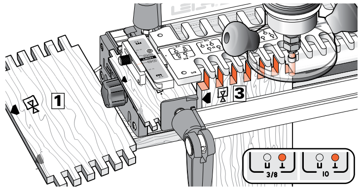
6-14 Rout both ends of boards 1 and 3 in position 1 . Be sure to keep the same edges to the side stop.
